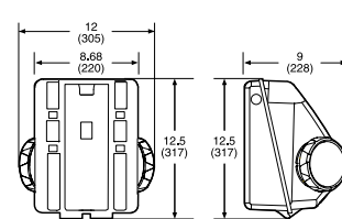
Carcasa Chica (16W-100W)
